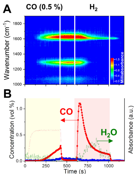
Fig. 5 Dynamic evolution of surface species elucidated by operando DRIFTS (A) during CO-CCR performed at 350^\circ\text{C} . Outlet gas composition (B) was obtained from averaging 5 cycles. CO blank signal (dotted line) obtained as average of 2 CCR cycles during a blank experiment at room temperature.
