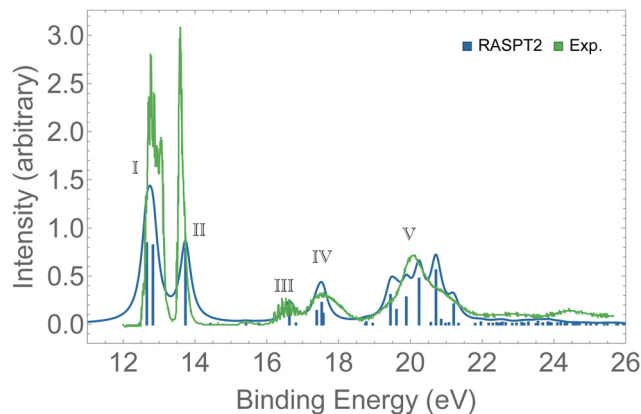
Fig. 2 PES of O_3 . The spectrum was shifted by +0.3 eV and broadened with Lorentzian functions with \text{fwhm} = 0.18 eV. For the assignments of the peaks, see Table 1.
