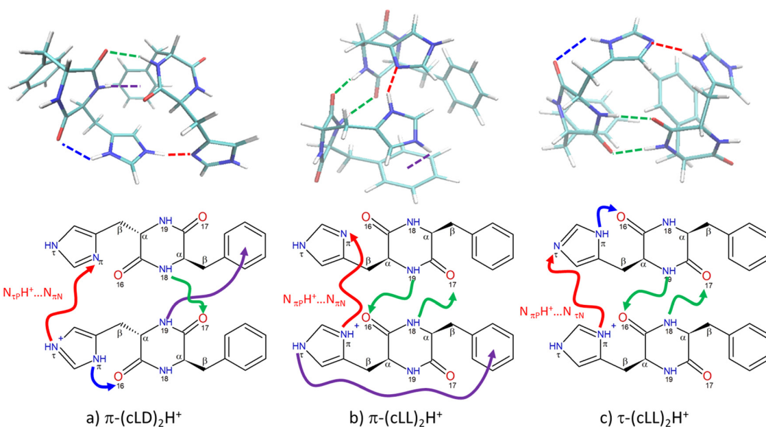
Fig. 2 Protonated dimers accounting for the experimental spectrum, calculated at the ri\text{-b97-d-D3BJ/def2-TZVPPD} level of theory. (a) \pi\text{-(c-LD)}_2\text{H}^+ , (b) \pi\text{-(c-LL)}_2\text{H}^+ , and (c) \tau\text{-(c-LL)}_2\text{H}^+ . Hydrogen bonds are indicated by dashed lines in the 3D structures (top) and by arrows in the 2D schemes (bottom). The strong ionic \text{NH}^+\cdots\text{N} interaction is shown in red, the neutral \text{NH}\cdots\text{O} interactions in green, the \text{NH}\cdots\pi interactions in purple, and the intramolecular \text{NH}\cdots\text{O} interaction in blue.
