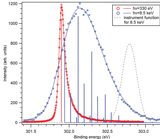
Fig. 1 The C 1s photoelectron spectrum from gas-phase \text{CF}_4 molecule, measured near the ionization threshold 29 (red) and in the HAXPES regime 18 (blue). The HAXPES spectrum is fitted using the recoil lineshape model. Excitations of vibrational levels are shown by vertical bars. The near-threshold spectrum shows no vibrational excitations, while the HAXPES spectrum is strongly modified by the recoil. Dashed curve shows the instrument function for the HAXPES measurement.
