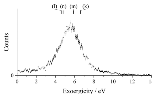
Fig. 10 Experimental exoergeticity spectrum for the reaction S^{2+} + N_2 \rightarrow S^+ + N_2^+ . The error bars represent two standard deviations of the associated counts. The literature exoergicities resulting from the pathways (k)–(n) are indicated. See text for details.
