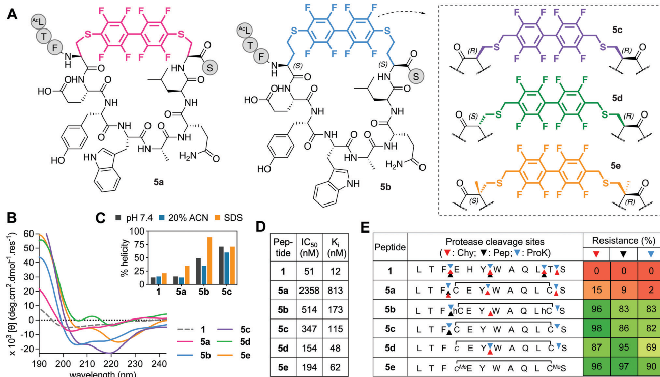
Fig. 5 A. Structures of perfluorobiphenyl ( i \rightarrow i + 7 )-crosslinked peptides 5a–e . B. CD spectra for 5a–e vs. 1 (50 \mu M) in 10 mM phosphate buffer (pH 7.4, 22 ^{\circ} C). C. Percent helicity calculated from CD spectra ( \theta_{220} ) in 10 mM phosphate buffer, 20% ACN or 20 mM SDS buffer ( 5d,e not helical). D. IC 50 = mean peptide concentration to inhibit 50% binding of fluorescent 1-FITC (10 nM) to hDM2 (25 nM) measured by FP. pIC 50 \pm SEM values are reported in Fig. S1 (ESI ^{\dagger} ). Binding affinity ( K_i ) calculated from IC 50 values. E. Heatmap indicating percent peptide intact after 2 h incubation with chymotrypsin (Chy), pepsin (Pep) or proteinase K (ProK) at 22 ^{\circ} C, pH 8 or 2 (Pep only), measured by LCMS. Arrows point to the respective cleavage sites as revealed by LCMS analysis of the cleaved fragments.
