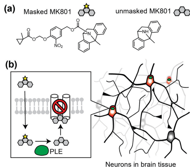
Fig. 14 Chemogenetic regulation of endogenous NMDAR using prodrug approach. (a) Chemical structure of a PLE-specific prodrug for NMDAR. (b) Schematic illustration of cell-specific inhibition of NMDAR using prodrug. The prodrug is converted into active inhibitor, MK801 to inhibit NMDAR in a cell-specific manner by PLE.
