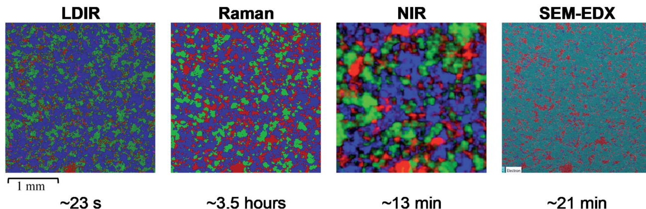
Fig. 5 (Left) LDIR, (left centre) Raman, (right centre) NIR and (right) SEM-EDX chemical images of the pharmaceutical tablet, where blue = microcrystalline cellulose, green = lactose monohydrate, red = hydrobromide salt API and magenta = croscarmellose sodium. For the SEM-EDX image cyan = MCC and lactose monohydrate as due to their chemical nature, they could not be individually identified. Each chemical image represents a 3000\ \mu\text{m} \times 3000\ \mu\text{m} area of sample and the total data collection time for each technique is displayed below the respective chemical image.
