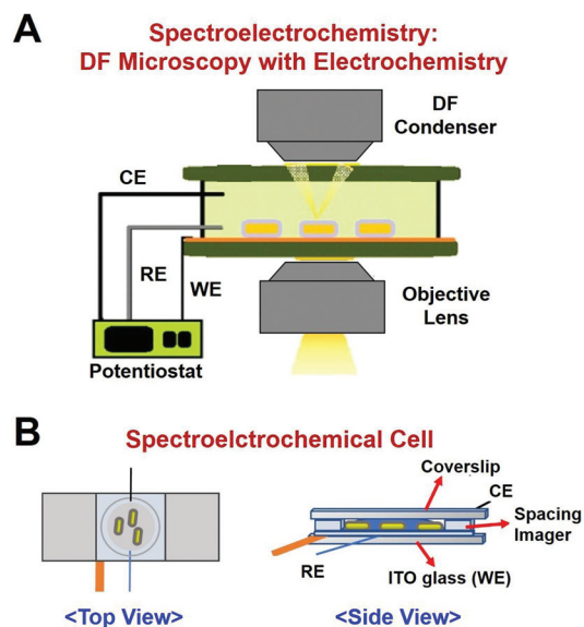
Fig. 2 (A) A schematic showing the experimental setup of the DF microscopy coupled with an electrochemical workstation. (B) Spectroelectrochemical cell diagram with ITO-coated glass as the working electrode (WE), Pt wire CE, insulated Pt quasi-reference electrode (RE), and spacing imager.
