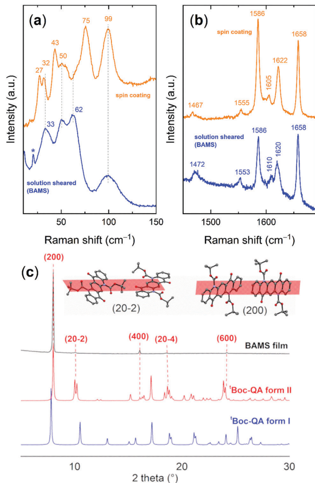
Fig. 6 (a) Lattice phonon and (b) intramolecular Raman spectra of spin cast and BAMS \beta Boc-QA films; (c) diffraction patterns of BAMS films and the two \beta Boc-QA polymorphs. Inset: Orientation of the two \beta Boc-QA molecules with respect of the (20-2) and (200) Miller planes in form II. H CH atoms omitted for clarity.
