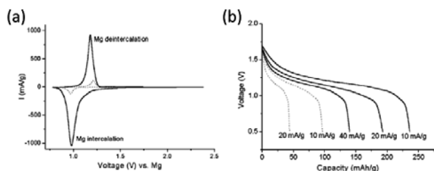
Fig. 16 (a) Cyclic voltammograms at 0.5 mV \text{s}^{-1} of \text{TiS}_2 nanotube (solid) and polycrystalline powder (dots) electrodes at 20 °C. (b) Discharge curves of \text{TiS}_2 nanotubes (solid) and polycrystalline \text{TiS}_2 (dots) at various current densities and 20 °C. Reproduced from ref. 159 with permission from The Royal Society of Chemistry.
