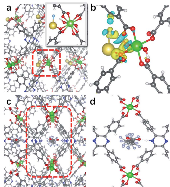
Fig. 5 (a) Optimized structure of NaF@In(tcpp), highlighting \text{Na}^+ and F^- interactions. (b) Charge density rearrangement upon formation of the bond at an isovalue of 0.002 \text{ eV } \text{\AA}^{-3} . (c) Binding of PFOA and In(tcpp) in PFOA@In(tcpp). (d) Configuration of PFOA@In(tcpp) (atoms are colored as follows: C grey, O red, N blue, In green, F light blue, Na yellow, H white).
