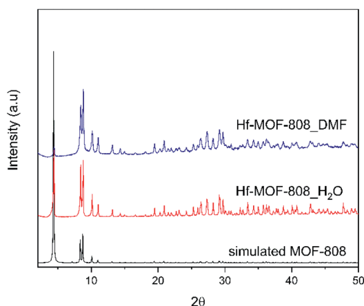
Fig. 1 Experimental and simulated PXRD patterns of Hf-MOF-808_ \text{H}_2\text{O} (red line) and Hf-MOF-808_ \text{DMF} (blue line).
