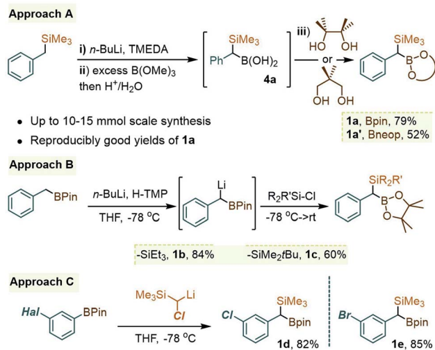
Scheme 2 Complementary deprotonation/quench approaches to the benzylic gem-Si/B core 1a . Approach A: (i) in hexane using 1.0 equiv. of n\text{-BuLi} at rt; (ii) with 3 equiv. of \text{B(OMe)}_3 , -78^\circ\text{C} to rt. Approach B: Li-TMP generated at -40^\circ\text{C} prior to addition of \text{BnBpin} at -78^\circ\text{C} . Approach C: lithiation of \text{Me}_3\text{SiCH}_2\text{Cl} with \text{sec-BuLi} /TMEDA followed by addition of Ar-Bpin.
