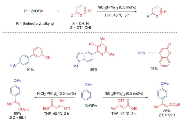
Scheme 12 Stereoselective nickel-catalyzed cross-couplings with organozinc pivalates.
