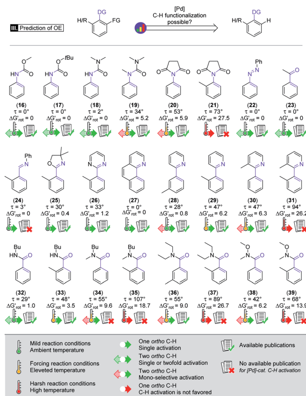
Scheme 4 Augmented demonstration and prediction of the steric repulsion and ortho effect. Values of \Delta G_{\text{rot}} are calculated at 25 °C. 30–46
