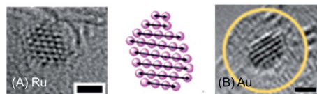
Fig. 4 Ruthenium and gold nanocrystals fabricated on a graphitic support by electron bombardment of \text{Ru}(\text{II}) and \text{Au}(\text{III}) complexes encapsulated in polymer micelles deposited on a lacey carbon EM grid in an aberration-corrected high-resolution transmission electron microscope. Interatomic distances: Ru–Ru 2.48 Å, Au–Au 2.73 Å. Scale bars 1 nm. Adapted from ref. 20 with permission from the Royal Society of Chemistry, copyright 2016. 20
