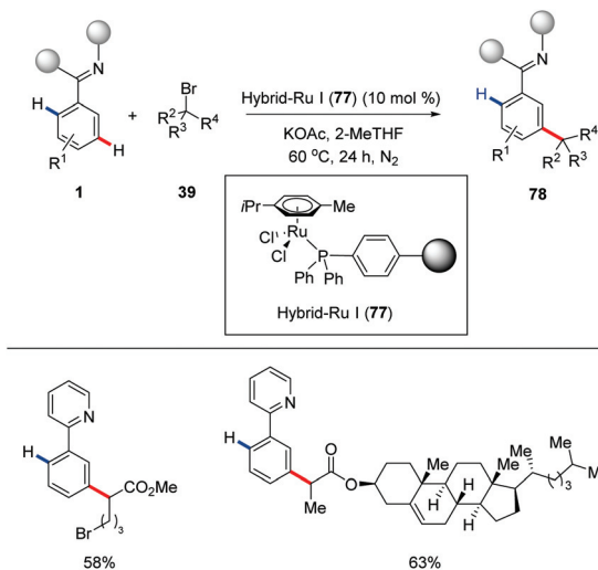
Scheme 27 meta -C–H Activation by recyclable hybrid-ruthenium catalysis.
