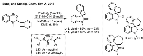
Scheme 15 Pd-Catalysed enantioselective C–H arylation.
