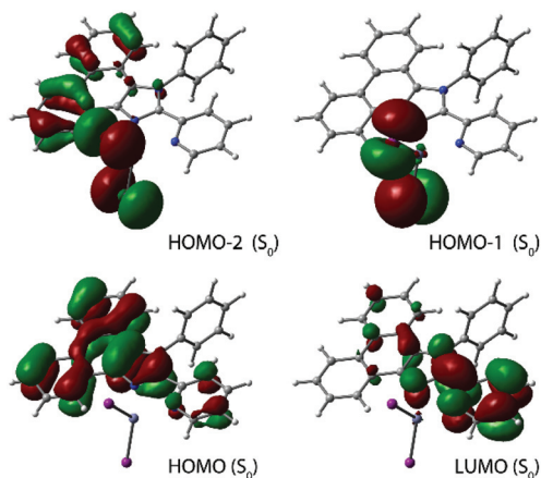
Fig. 3 Frontier molecular orbitals for the ground states of complex 11 (in chloroform, the singly occupied orbitals for S_1 and T_1 states are shown in Fig. S4†).
