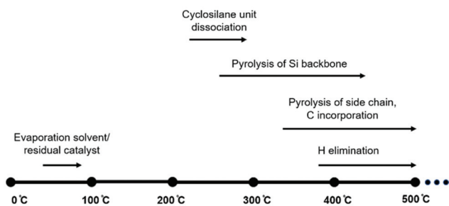
Fig. 6 Proposed polycyclosilane pyrolysis.
