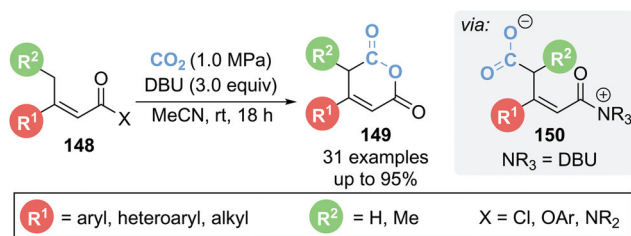
Scheme 32 The use of \text{CO}_2 as C(1) building block in the synthesis of glutamic anhydride.
