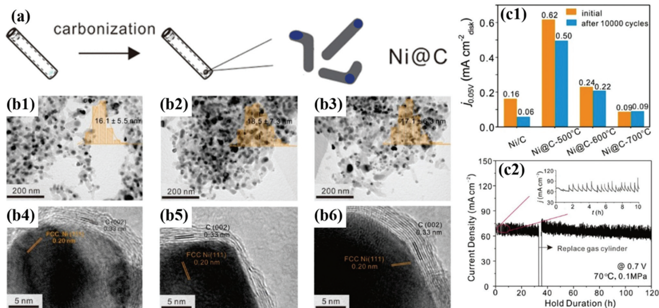
Fig. 11 (a) Synthesis diagram of the Ni@C catalyst. (b1–3) TEM images of Ni@C with the inset showing the particle sized distribution histogram. (b4–6) HR-TEM images of Ni@C showing carbon shell thickness for Ni@C-500, Ni@C-600, and Ni@C-700, respectively. (c1) Current densities of Ni@C catalysts before and after ADT (10 000 cycles). (c2) Stability test at 0.7 V for 120 h under single cell conditions at 70 °C with fully humidified H 2 and O 2 fed at the anode and cathode, respectively, with permission from ref. 56, ACS copyright 2020.
