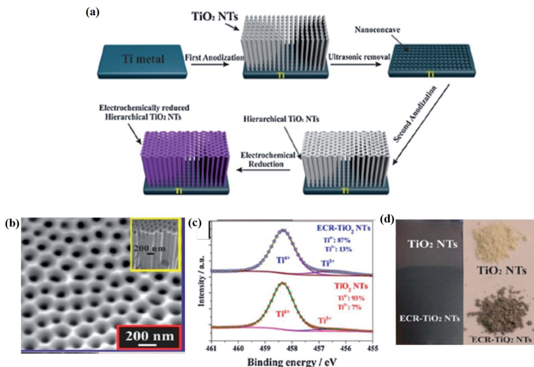
Fig. 11 (a) Schematic representations of the anodization process, along with the electrochemical reduction procedure for the formation of self-doped \text{TiO}_2 nanotubes. (b) SEM image of the electrochemically reduced nanotubes. (c) XPS spectra of Ti 2 p_{3/2} . (d) Digital image of the samples before and after the anodization process. Reprinted with permission from ref. 85. Copyright 2013, Royal Society of Chemistry.
