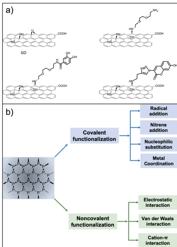
Fig. 1 Functionalisation routes used for the preparation of GO and NBP nanoplatforms. (a) The versatile approach of the epoxide opening reaction with primary amines (reproduced from ref. 16 with permission from IOPscience, copyright Creative Commons Attribution 3.0 licence 2018). (b) Strategies for functionalisation of BP (reproduced from ref. 17 with permission from Wiley, copyright Creative Commons Attribution 3.0 licence 2019).
