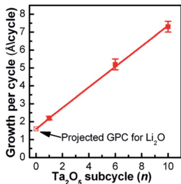
Fig. 9 The GPC of the lithium tantalate thin films as a function of Ta 2 O 5 subcycle number, using pulsing sequences of 1 \times \text{Li}_2\text{O} + n \times \text{Ta}_2\text{O}_5 ( n = 1, 6, \text{ and } 10 ). 29
