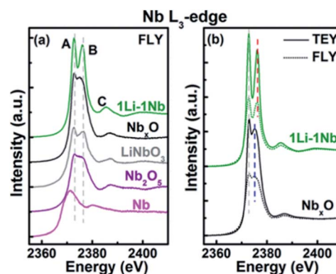
Fig. 11 Nb L 3 -edge XANES spectra: (a) fluorescence yield (FLY) XANES spectra of ALD thin films and standard powders (LiNbO 3 , Nb 2 O 5 , and Nb) and (b) total electron yield and FLY XANES spectra of 1Li-1Nb and Nb x O thin films. 32
