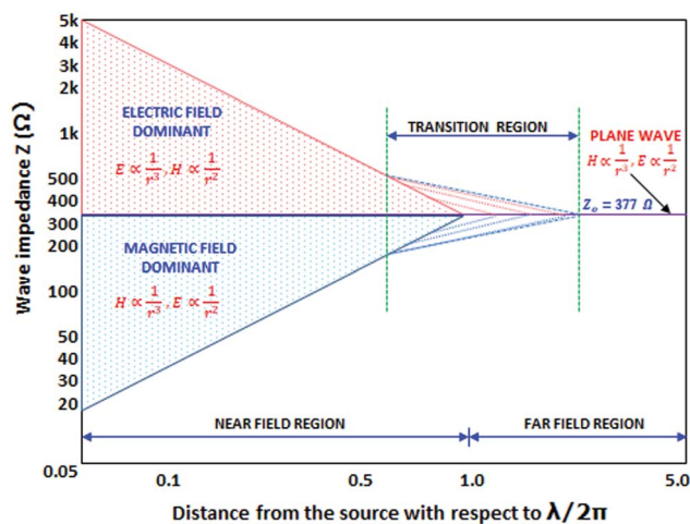
Fig. 2 Dependence of the wave impedance on the distance from the source normalized to \lambda/2\pi (modified from ref. 24 with permission from Intech, copyright 2012).
