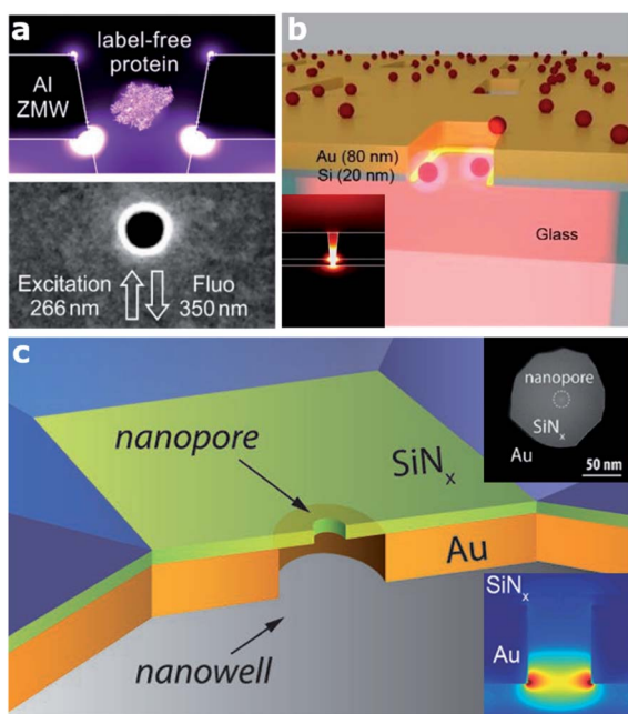
Fig. 1 Various architectures of zero mode waveguide (ZMW) plasmonic nanoapertures. (a) Deep ultraviolet plasmonic enhancement of single protein autofluorescence in an Al ZMW. This figure has been reproduced from ref. 31 with permission from ACS Publications, copyright 2019. (b) A hybrid Au–Si zero mode waveguide for enhanced single molecule detection. This figure has been reproduced from ref. 30 with permission from the Royal Society of Chemistry, copyright 2019. (c) Enhanced single molecule fluorescence detection with a plasmonic nanowell–nanopore device architecture made of a nanowell fabricated in a gold film (orange) with a nanopore drilled in a freestanding \text{Si}_3\text{N}_4 membrane (light green). This figure has been reproduced from ref. 40 with permission from Wiley, copyright 2017.
