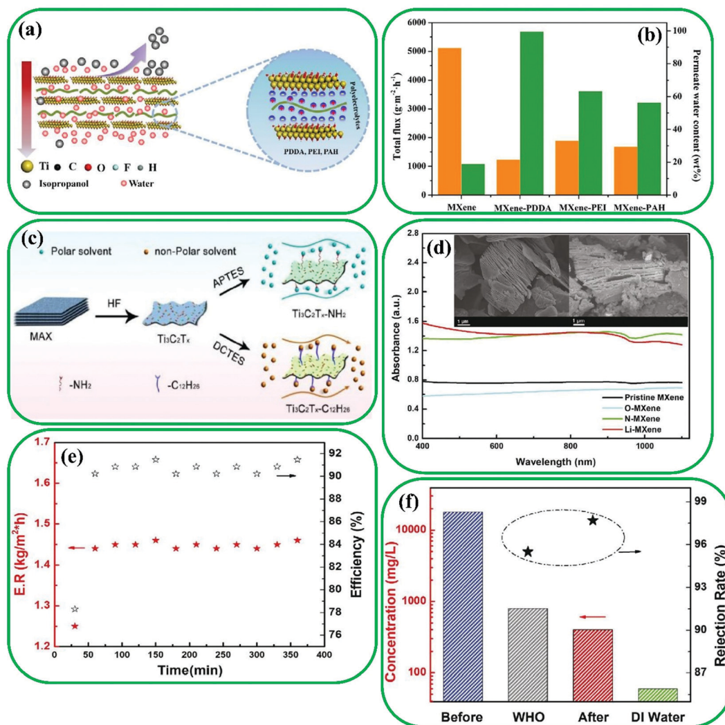
Fig. 21 (a) Schematic illustration of Ti_3C_2 laminar membranes functionalized via polyelectrolytes. (b) Effects of polyelectrolytes on MXene-based membranes for pervaporation dehydration of 90 wt% isopropanol/water at 50 °C. Reproduced with permission. 250 Copyright 2020, American Chemical Society. (c) Synthesis process of pristine Ti_3C_2 and functionalized Ti_3C_2 composites. Reproduced with permission. 253 Copyright 2017, Elsevier. (d) UV-vis absorbance spectrum of various powders. Inset: SEM images of MXene flakes, pristine MXene (left) and Li-MXene (right). (e) Energy conversion efficiency evaluation during continuous 6 h illumination. (f) Salt rejection rate revealed by ion concentration comparison before and after desalination showing the capability to produce drinking water. Reproduced with permission. 254 Copyright 2020, Wiley.
