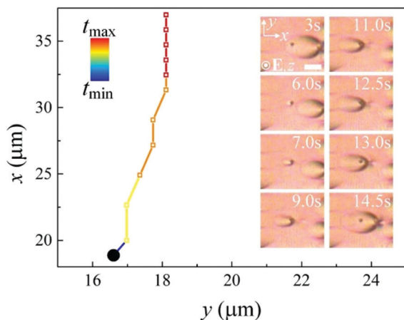
Fig. 9 Trajectory of a swallow-tail soliton nucleated from a micro-particle. The color bar represents the elapsed time. t_{\text{min}} = 0 s, t_{\text{max}} = 17.5 s, time interval \Delta t = 0.5 s. Insets are time series of micrographs of the nucleation of a soliton at a micro-particle. U = 7.6 V, f = 10 Hz, T = 33.5 °C, scale bar 10 \mu\text{m} , micro-particle diameter R_p = 1.5 \mu\text{m} .
