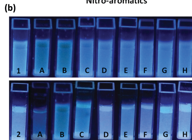
Fig. 3 (a) Fluorescence quenching (%) of 1 and 2 dispersed in water (1 mg, 2 mL) by different NACs (200 μL, 1 mM). (b) Cuvette photographs of 1 and 2 before and after the addition of 200 μL of different analytes upon UV-light illumination at \lambda = 365 nm, where, A: TNP; B: 2,4-DNP; C: 4-NP; D: 2,4-DNT; E: TNT; F: 2,6-DNT; G: 1,3-DNB; H: NB.
