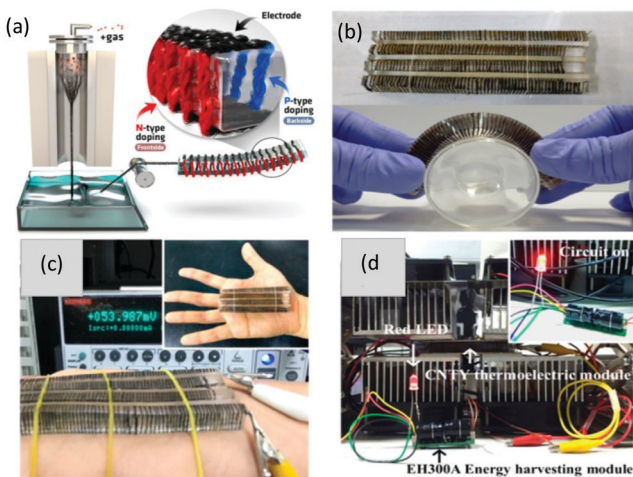
Fig. 6 (a) Fabrication process of the CNT and flexible TE device. (b) Picture showing the flexibility of the fabricated TEG. (c) Output voltage obtained from the TEG using body heat. (d) Image of a red LED powered using the flexible TEG at \Delta T = 50 K. Reprinted with permission from ref. 20 (J. Choi, Y. Jung, S. J. Yang, J. Y. Oh, J. Oh, K. Jo, J. G. Son, S. E. Moon, C. R. Park, H. Kim, 11 (2017) 7608–7614). Copyright (2017) ACS Publications.
