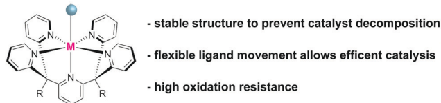
Chart 5 Summary of features of water oxidation catalysts with PY5 -type ligands.
