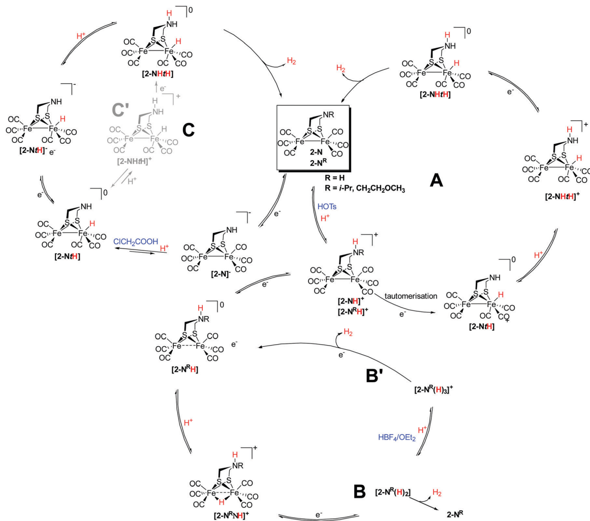
Fig. 99 Catalytic pathways for the proton reduction by \text{Fe}_2(\text{adt})(\text{CO})_6 and \text{Fe}_2(\text{adt}^{\text{R}})(\text{CO})_6 analogues with acids of varying strength.
