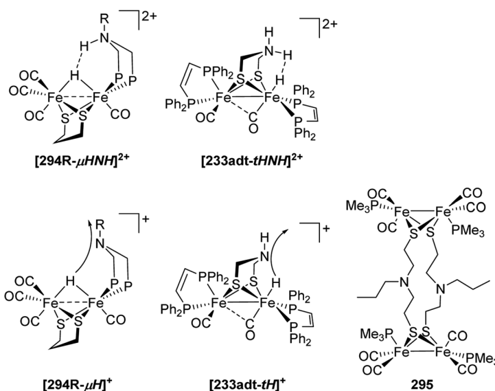
Fig. 93 Top: H–H interaction in double-protonated complexes. Bottom: Deprotonation of hydride complexes and structure of complex 295 (Note: P = PPh 2 in 294R ).
