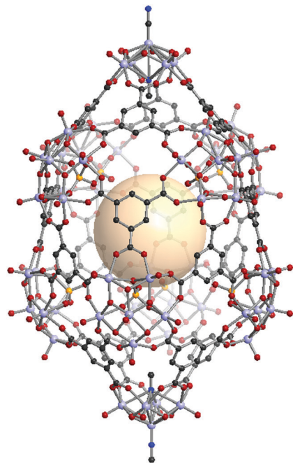
Fig. 35 Structural illustration of VMOP-24, \{[V_5O_9(CN)_2]_2[V_6O_{11}(SO_4)_8]\}(\text{C1})_{16} . 161
