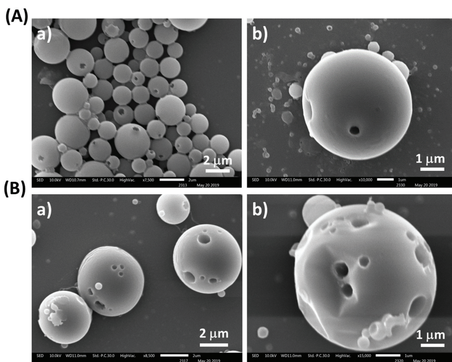
Fig. 5 (A) (a) SEM analysis demonstrating the opening of NB-shell-pores at pH 5. (b) Zoomed image of the pore opening at pH 5. (B) (a) At pH 2, multiple pores were formed on the NB-shells as is evident in the figure and (b) zoomed image of the porous NB-shells observed at pH 2.
