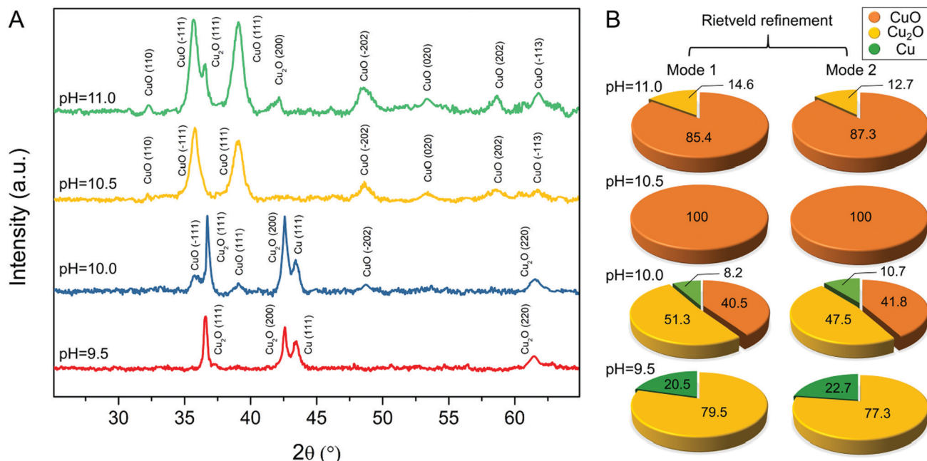
Fig. 4 Phase identification analysis of the Cu x O products exfoliated from the surface of liquid metal. (A) XRD patterns. (B) Rietveld phase quantification results.
