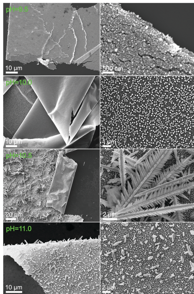
Fig. 6 Morphological analysis of the \text{Cu}_2\text{O} sheets obtained at different pH. Samples were exfoliated from the bulk liquid metal on the Si wafer.
