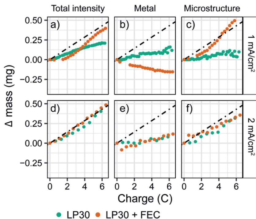
Fig. 3 The fitted intensities of the in situ NMR spectra of Li metal for constant currents of (a–c) 1 \text{mA cm}^{-2} and (d–f) 2 \text{mA cm}^{-2} in the two electrolytes LP30 (green) and LP30 + FEC (orange). The dashed line indicates m_{\text{echem}} , the calculated mass deposited according to the current passed by the electrochemistry.
