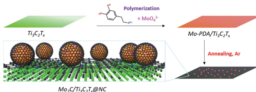
Fig. 1 Synthetic illustration of the preparation of \text{Mo}_2\text{C}/\text{Ti}_3\text{C}_2\text{T}_x@\text{NC} .
