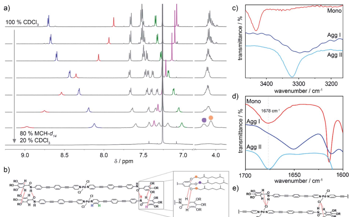
Fig. 4 (a) Development of the ^1\text{H} NMR resonances of ( R )-1 upon self-assembly into Agg I , induced by decreasing solvent polarity from 100% \text{CDCl}_3 (monomer) to 20% \text{CDCl}_3/80\% \text{MCH-}d_{14} ( c = 2 \times 10^{-3} M). (b) Parallel molecular packing governed by amide-to-amide hydrogen bonding and unconventional \text{C-H}\cdots\text{O}_{\text{alkoxy}} interactions, which are illustrated in the zoom. Right panel: partial FT-IR spectra of monomer ( \text{CHCl}_3 , c = 0.5 mM), Agg I and Agg II (both thin films), showing regions of N–H (c) and carbonyl \text{C=O} (d) stretching frequencies. (e) Excerpt of the molecular packing in Agg II illustrating the \text{N-H}\cdots\text{Cl} interactions leading to a slipped molecular arrangement.
