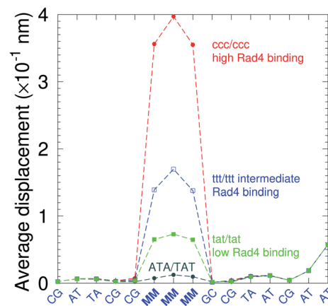
Fig. 11 Average displacements of the sequences with central triple mismatches, ccc/cc c (red bullets), ttt/ttt (blue squares), tat/tat (green boxes) and their reported Rad4 binding specificities. 11 For comparison, a sequence without a mismatch is also shown (grey bullets). The calculation was carried out at 150 K, which has no relation to the melting temperatures. Sequences are TGACTCGA-CATCCMMMGCTACAA/ACTGAGCTGTAGCMMMGATGTT based on ref. 11 and, only the central part around the mismatched region MMM/MMM is shown.
