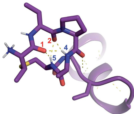
Fig. 11 View of the hydrogen bonding network present in ring A of CyLL_5^L that contributes to preorganization of the substrate to form the L stereochemistry. Hydrogen bond donor residue numbers are in blue font, while hydrogen bond acceptor residue numbers are in red font.
