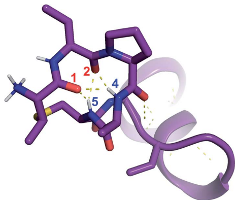
Fig. 11 View of the hydrogen bonding network present in ring A of \text{CyLL}_5^{\text{L}} that contributes to preorganization of the substrate to form the \text{L} stereochemistry. Hydrogen bond donor residue numbers are in blue font, while hydrogen bond acceptor residue numbers are in red font.
