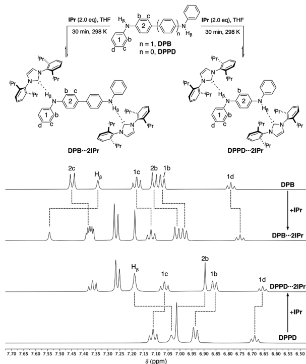
Fig. 4 Partial ^1\text{H} NMR spectra (500 MHz, \text{THF}-d_6 ) of DPB (50 mM), \text{DPB}\cdots 2\text{IPr} , \text{DPPD}\cdots 2\text{IPr} , and DPPD (50 mM). Dashed lines highlight the chemical shift changes upon hydrogen bonding to IPr.
