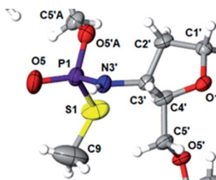
Fig. 1 Crystal structure of {}^{DMT}dG^{iBu}_{NPSMe}T_{OAc} 10f showing partial structure and spatial orientation of substituents around the phosphorus stereogenic center (marked P1). Compound 10 was obtained from the monomer 6Gf (fast-eluting 5'- O -DMT-3'-amino-2',3'-dideoxy- N - i Bu-guanosine-3'- N -(2-thio-4,4-pentamethylene-1,3,2-oxathiaphospholane). The oxygen atom marked O5'A belongs to the thymidine residue.
