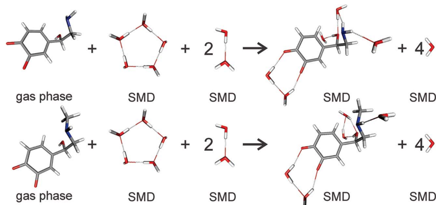
Fig. 2 Scheme of noradrenaline o-quinone (top) and adrenaline o-quinone (bottom) interacting with water molecules to calculate the solvation free energy. Analogous schemes were used to calculate the solvation free energies for all protonation states.
