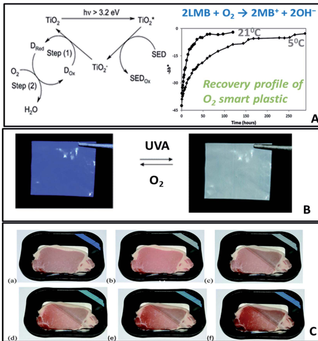
Fig. 16 (A) Mechanism of a UVA-activated O 2 indicating plastic, comprising a semiconductor TiO 2 photocatalyst, a redox dye ( D ox , such as methylene blue) and a sacrificial electron donor (SED, such as DL-threitol). (B) Photographs of a section of extruded O 2 -indicator film (a) before photoactivation and (b) after 90s exposure to UVA. (C) Photographs of pork, packaged within an O 2 smart plastic film, heat sealed to the inside of a PET packaging lid. The package was sealed in the absence of oxygen (a) and the indicator activated (b). The packaging lid was then broken and partly lifted back, and photographed immediately (c), and after 1 day (d), 2 days (e) and 4 days (f) in a fridge at 5 °C. Adapted from ref. 160 with permission from The Royal Society of Chemistry, 2012.
