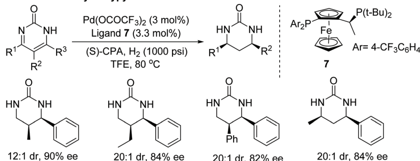
Fig. 43 Palladium catalysed AH of mono- and disubstituted 2-hydroxypyrimidines.
