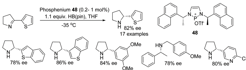
Fig. 62 Phosphonium cation-catalysed ATH of cyclic imines.
