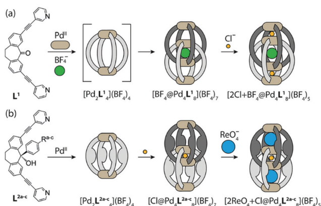
Fig. 16 Synthesis of interpenetrated dimer cage: (a) [Pd_4L_8 \cdot BF_4] with BF_4^- as a template anion and Cl^- anions in the outer pockets, (b) [Pd_4L_8 \cdot Cl] with Cl^- as a template anion and ReO_4^- in the outer pockets. Reproduced with permission from ref. 73. Copyright 2013, American Chemical Society.
