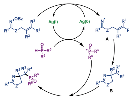
Scheme 20 Proposed mechanism.
