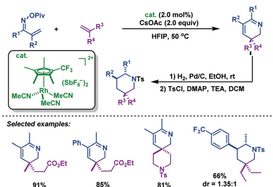
Scheme 49 Rovis' Rh(III)-catalyzed coupling of \alpha,\beta -unsaturated oxime esters with 1,1-disubstituted alkenes for the synthesis of 2,3-dihydropyridines.
