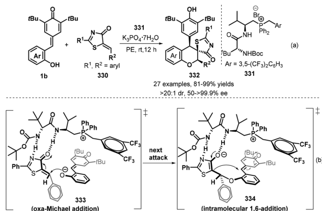
Scheme 74 Enantioselective construction of chroman-thiazolones.
