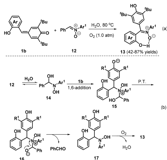
Scheme 4 \text{H}_2\text{O} -Mediated reaction of p -QMs with nitrones.
