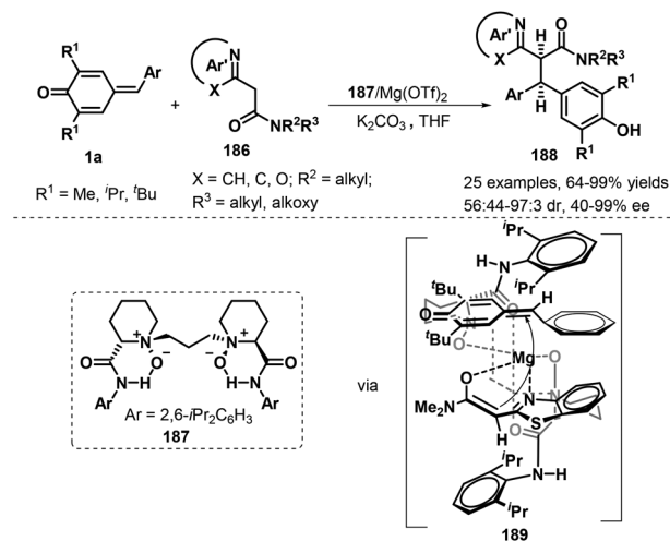
Scheme 39 1,6-Addition of 2-azaarylacetamides to p -QMs.
