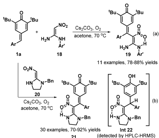
Scheme 5 Synthesis of \beta -nitroenamine derivatives.
